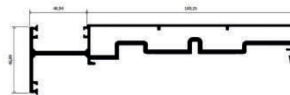
Marco Vertical 4"
