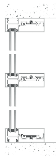
Ensamble Vertical
