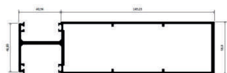
Marco Vertical 6"
